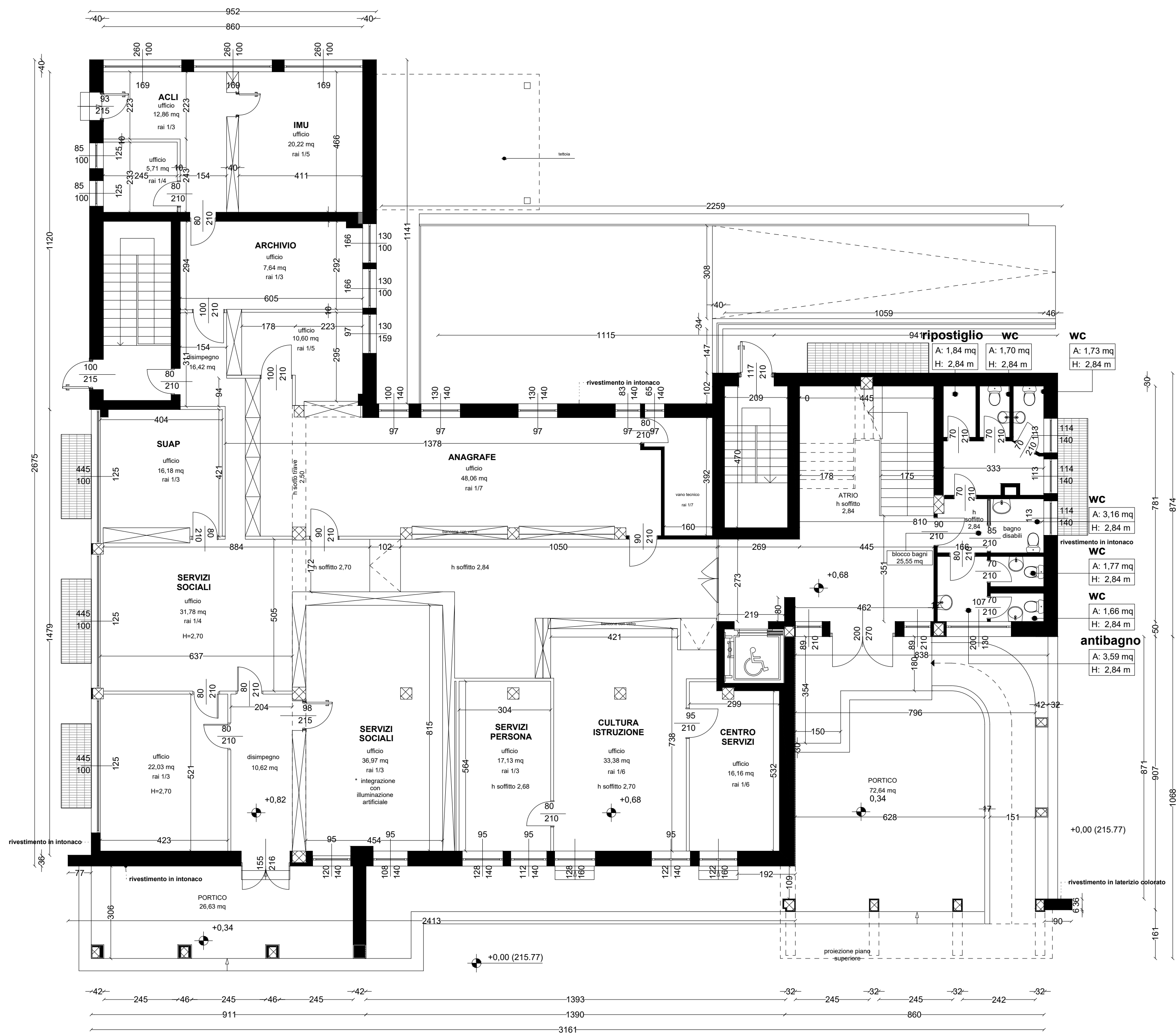
PIANO TERRA scala 1:100
